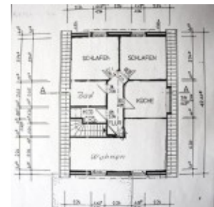
Grundriss FeWo
